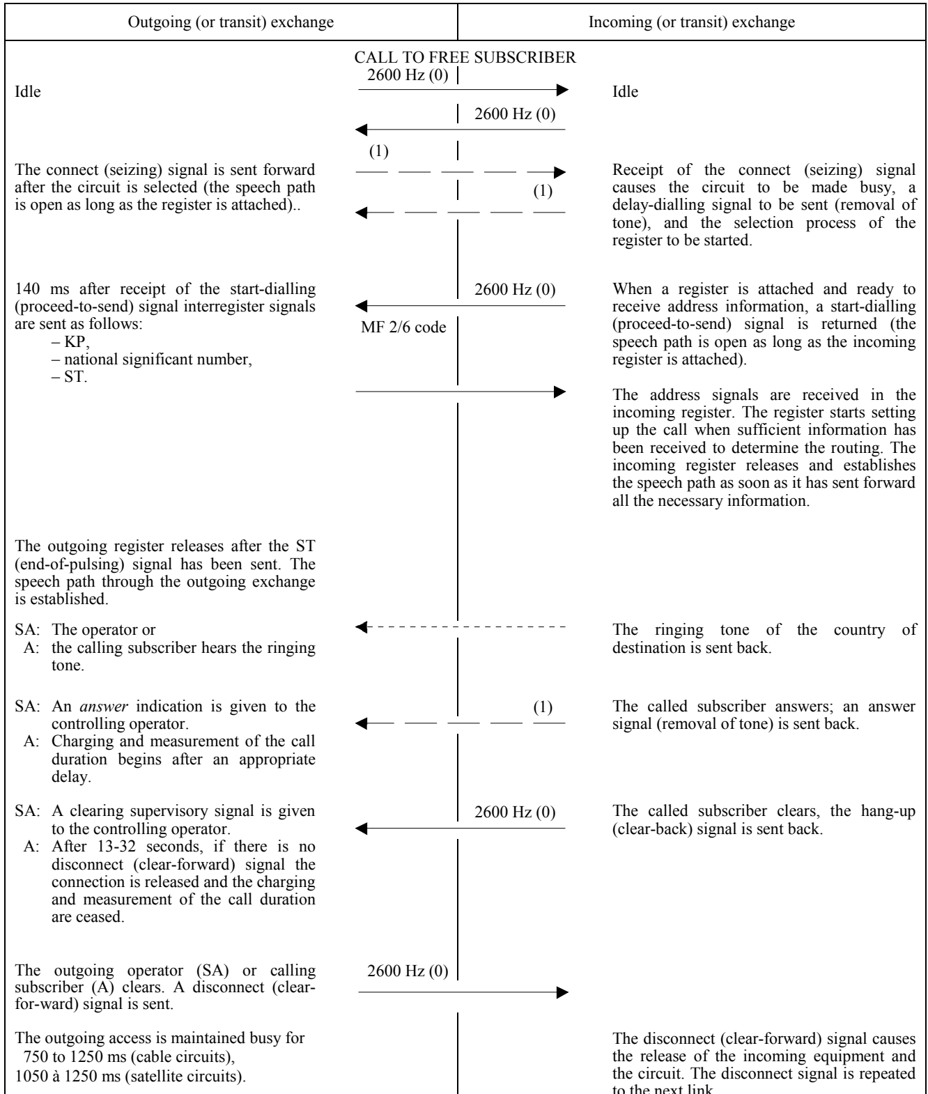
Semi-automatic (SA) and automatic (A) traffic in Zone 1
