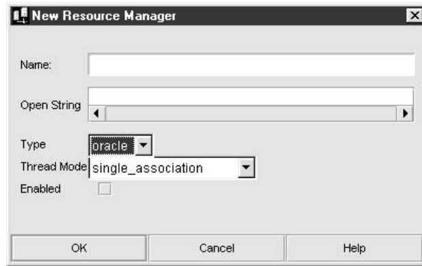
FIGURE 33-18 Adding a resource manager
