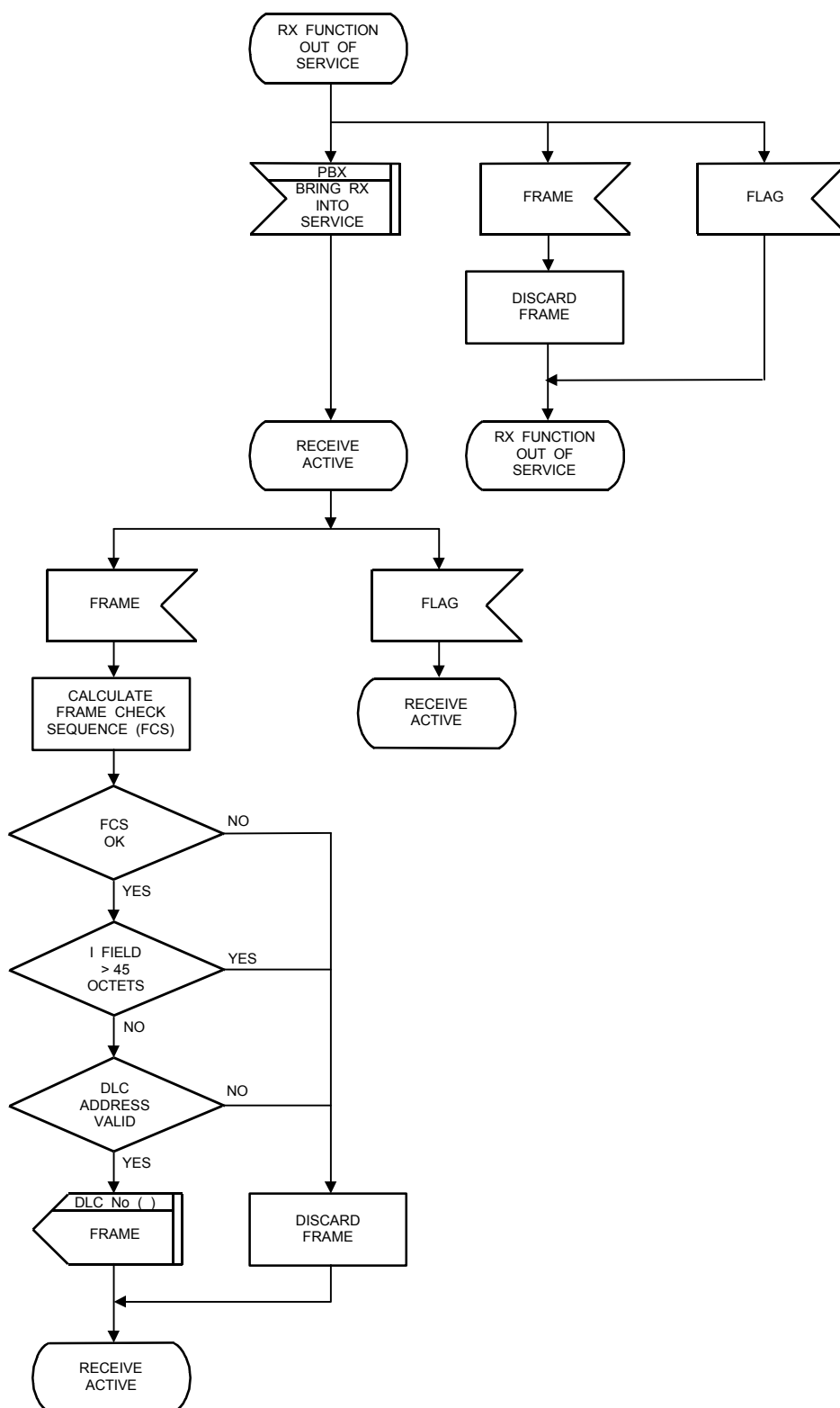
DPNSS 1 LAYER 2: RECEIVE FUNCTION FIG.1 (DPNSS[188] SECTION 3)
