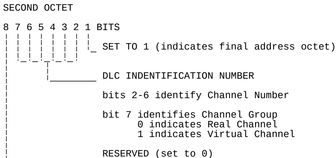
Figure 2b - Address Field Coding (Second Octet)
